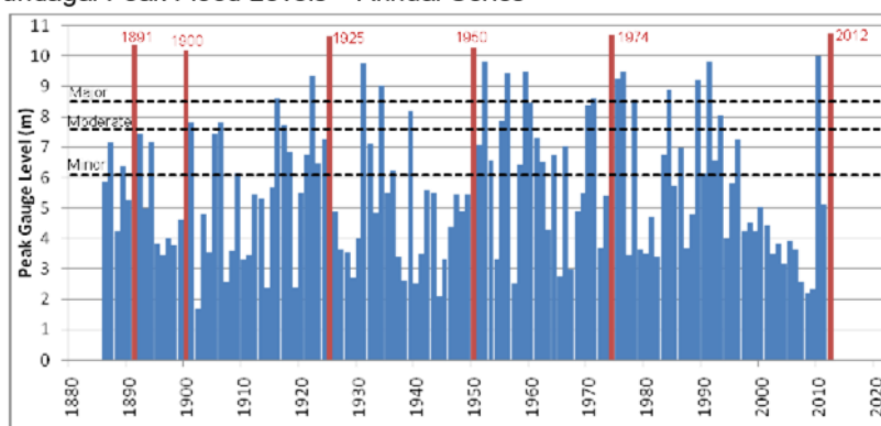
Chart 1: Gundagai Peak Flood Levels – Annual Series
