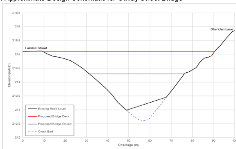
Diagram 8: Approximate Design Schematic for Otway Street Bridge
