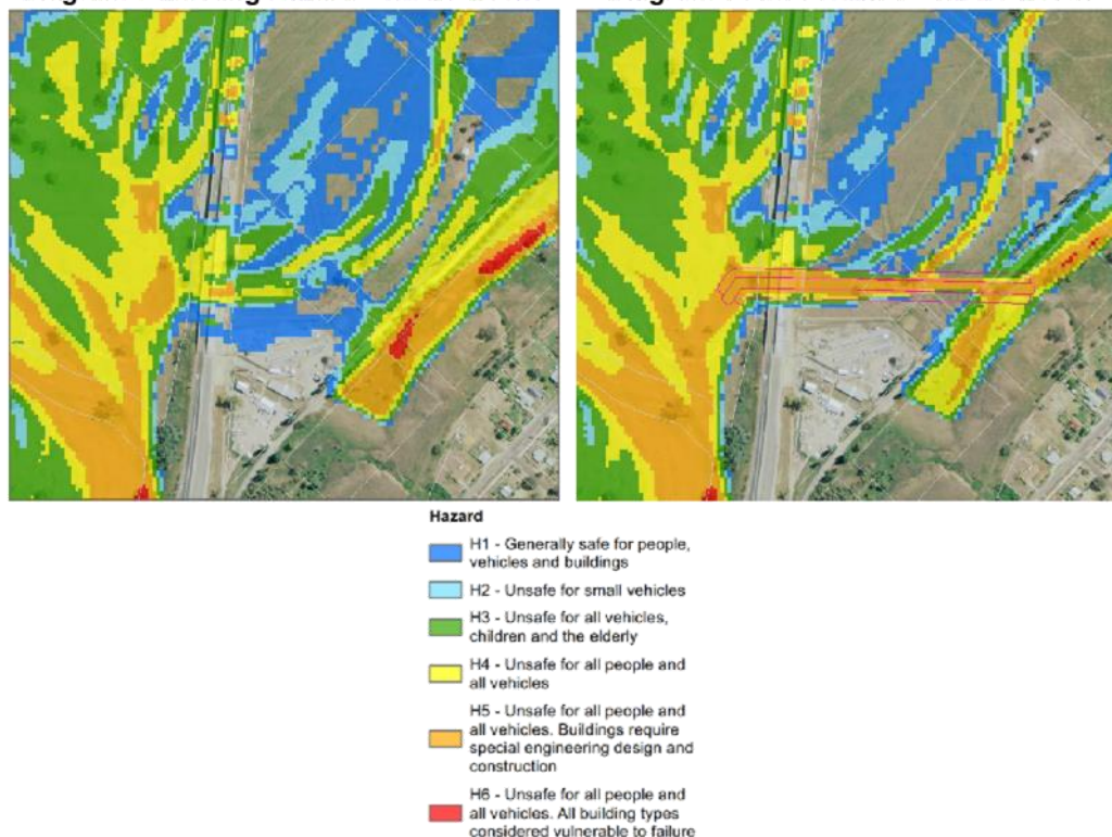
Diagram 5 Existing Hazard - 0.2 EY Event
